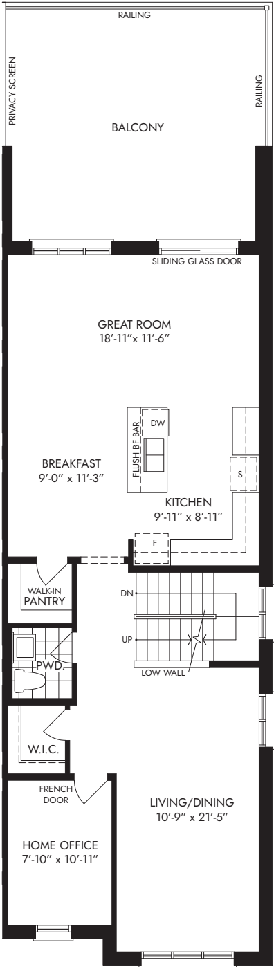
MAIN FLOOR ELEV. A
